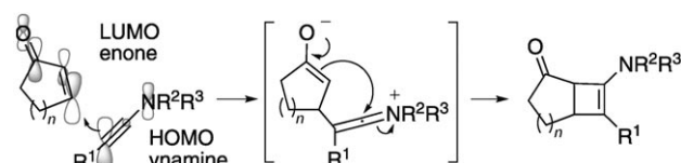
Scheme 1. The original Ficini reaction with ynamines.
